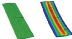
Reden's modelling strategy for TenCate's artificial turf starts on a micro level with Abaqus FEA analysis of an individual synthetic fiber, shown here. Mass, shape, bendability, height and other characteristics can be modified and retested until the desired requirements are met.
